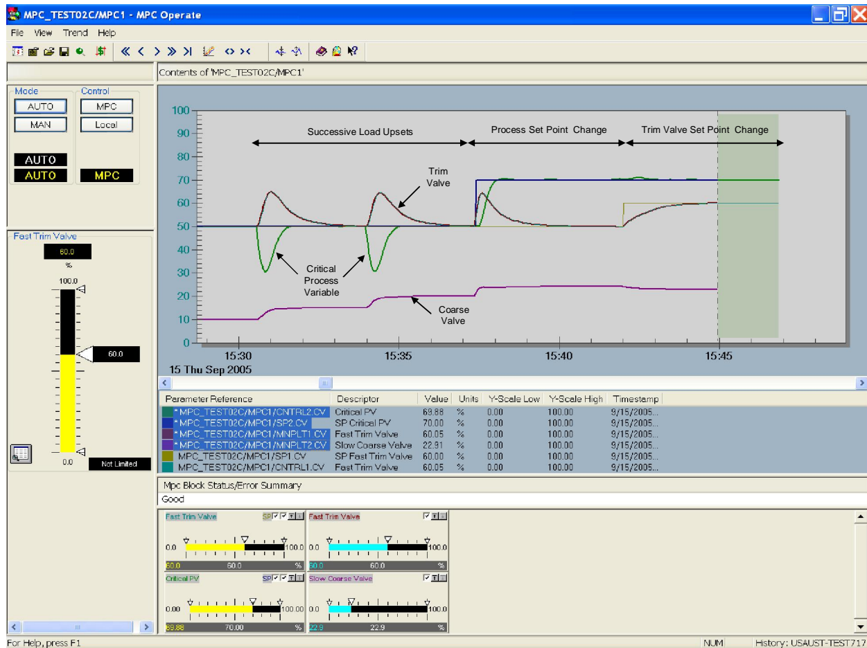
Figure 6 Trend in MPC Operate of response of DeltaV Predict to disturbances and setpoints
