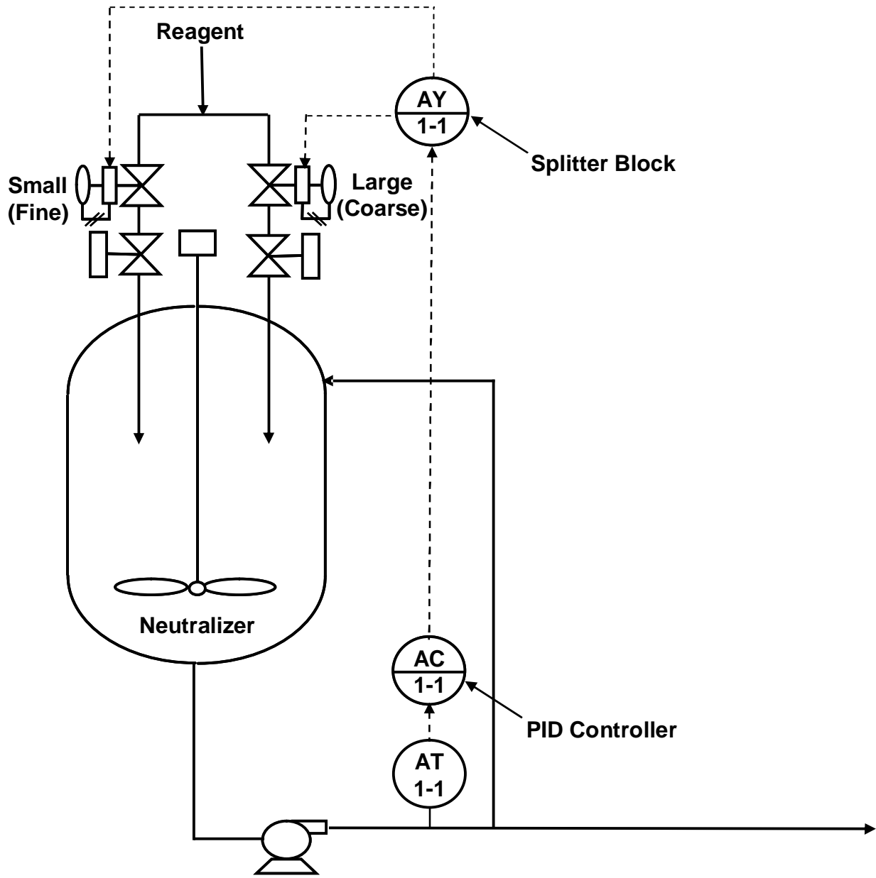
Figure 1 Split-range control for a neutralizer
