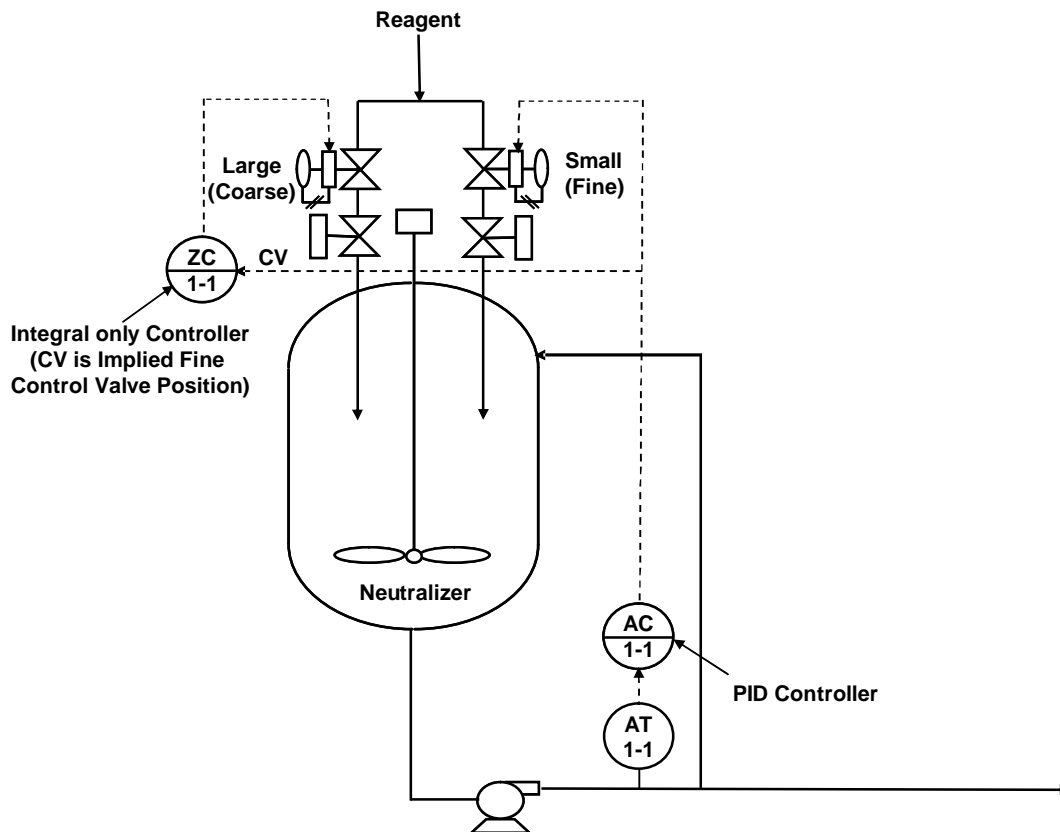
Figure 2 Valve position controller for a neutralizer
